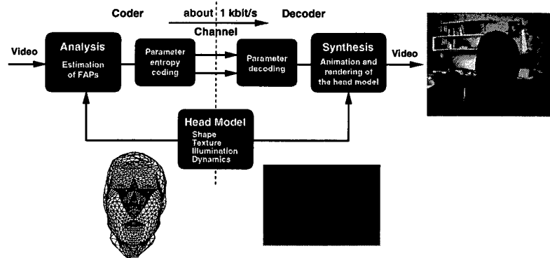
Figure 1: Basic structure of the model-based codec.
