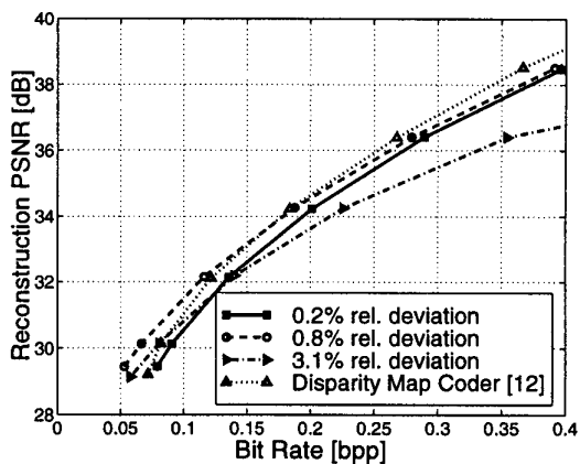
Figure 9: Rate-Distortion curves for different model resolutions if geometry bit-rate is taken into account.
