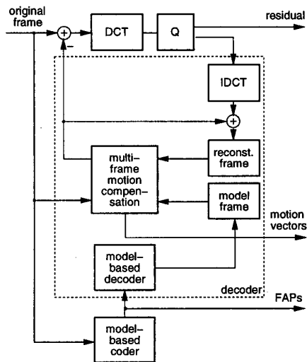
Figure 2: Structure of the proposed "model-aided" video coder. Traditional block-based MCP from the previous decoded frame is extended by prediction from the current model frame.
